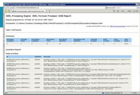
Formula Generator
