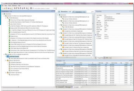
Taxonomy Explorer
