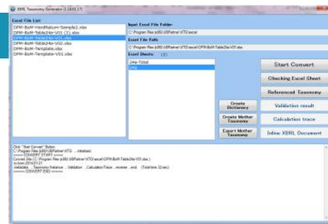
Taxonomy Generator
